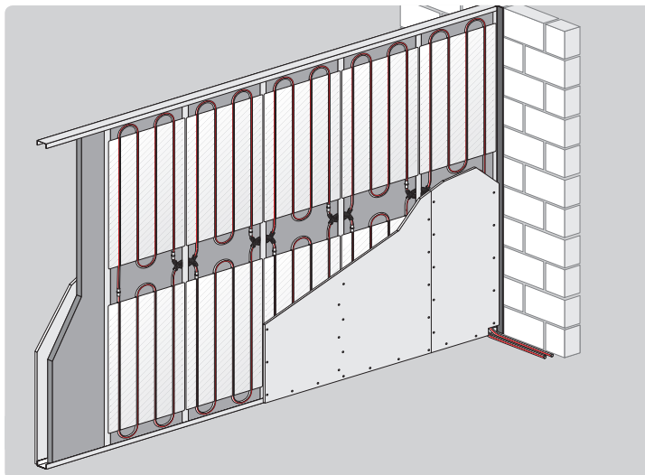
Uponor Siccus SW in serieschakeling
